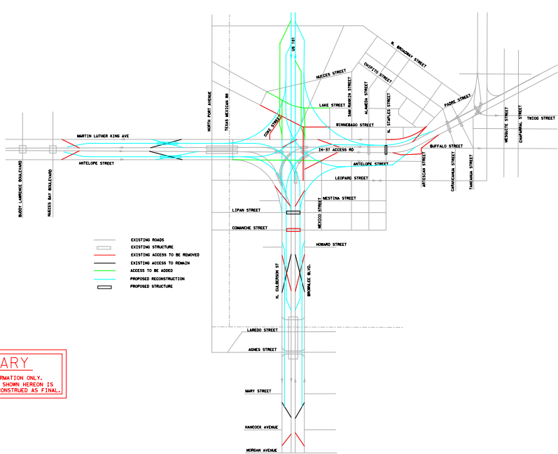
PROPOSED TRAFFIC ACCESS DIAGRAM
